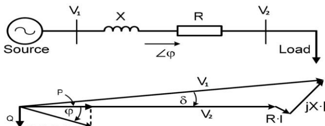
Figure 2: Power System without Compensation.
