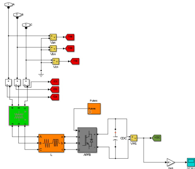
Figure 10: D-STATCOM Model.
