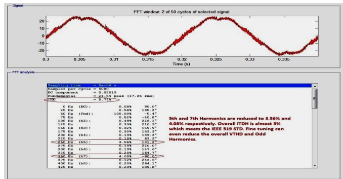
Figure 21: FFT analysis for Current wave form with D-STATCOM based on Park's Transformation technique.
