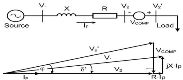
Figure 4: Series Compensation for power system.
