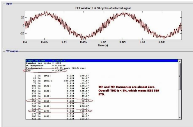
Figure 19: FFT analysis for Current wave form with D-STATCOM based on generalized technique.
