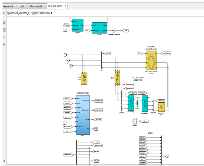
Figure 9: Matlab /Simulink Model for DFIG.
