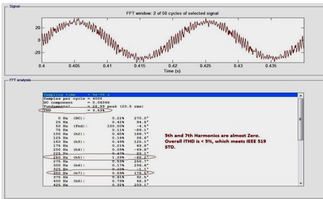
Figure 18: FFT analysis for Voltage wave form with D-STATCOM based on generalized technique.
