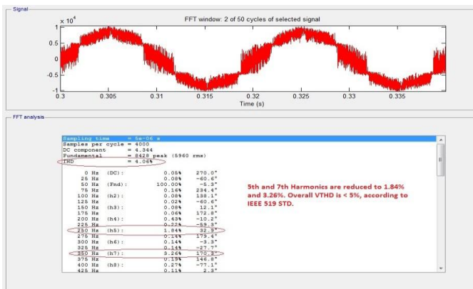
Figure 20: FFT analysis for Voltage wave form with D-STATCOM based on Park's Transformation technique.
